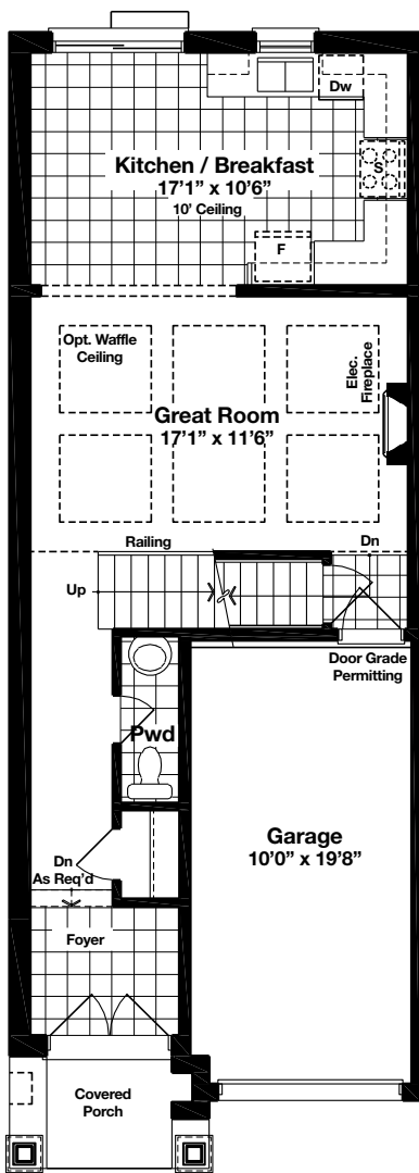
MAIN FLOOR Elev. A
