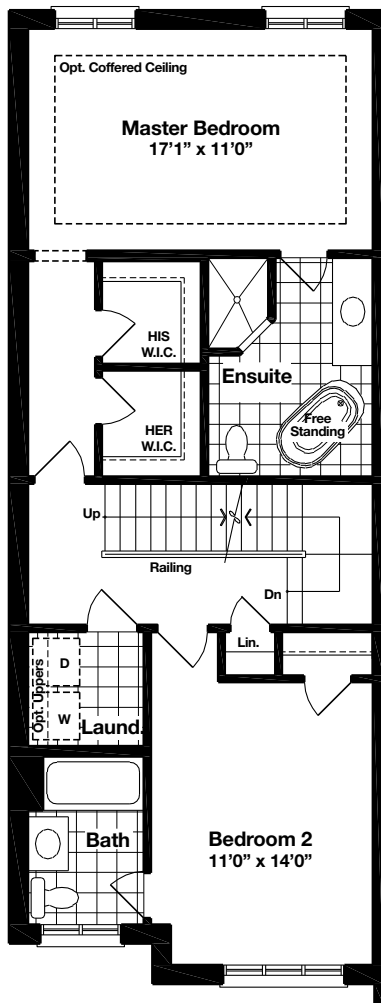
UPPER FLOOR Elev. A
