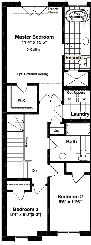
UPPER FLOOR Elev. A
