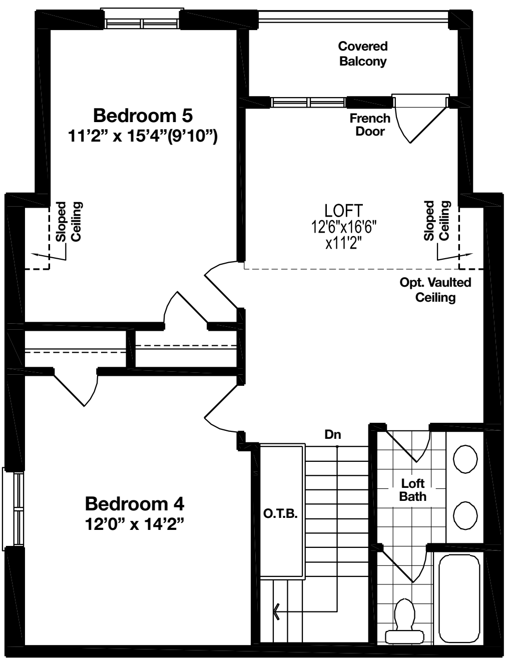
LOFT FLOOR Elev. A, B & C
