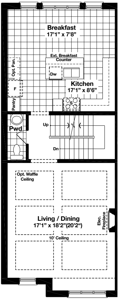
MAIN FLOOR Elev. A
