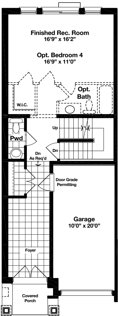
GROUND FLOOR Elev. A
