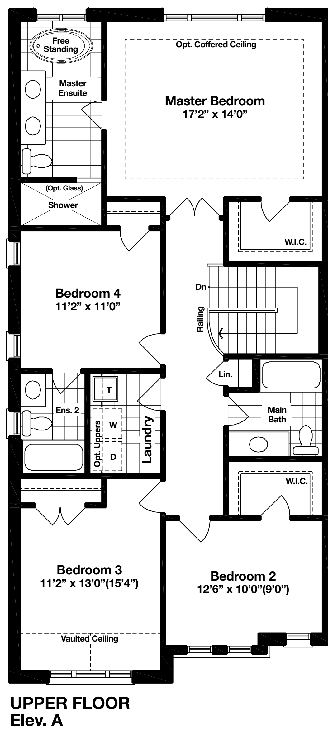
Elevation A - 2,440 sq. ft.
